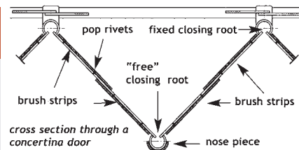
Nose pieces for Concertina Doors
