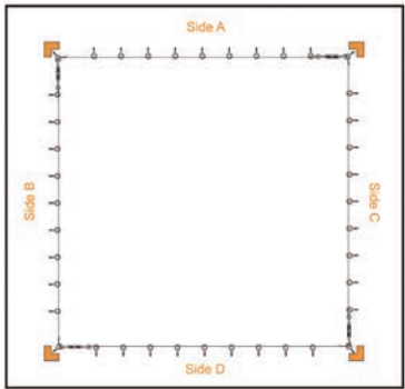
Attach one end of the wire rope to a corner fixing using a loop of wire and secure with either 2 ferrules (each crimped twice) or 2 wire rope grips.
