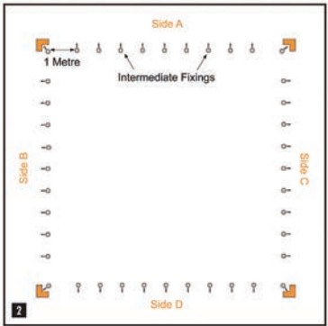
Drill holes and fit intermediate fixings at 1 m intervals in a straight line between the corner fixings.
